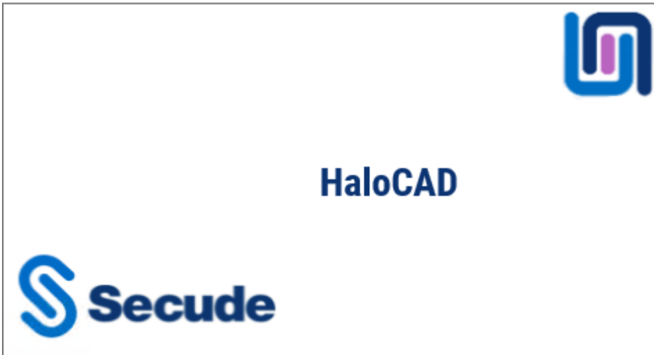
Startup dialog
