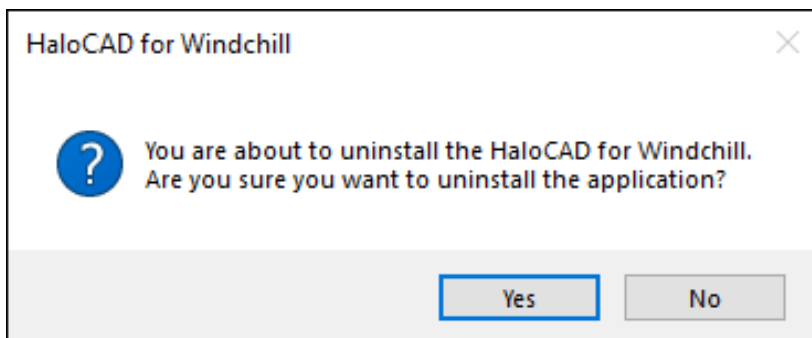
Uninstall Message #1
